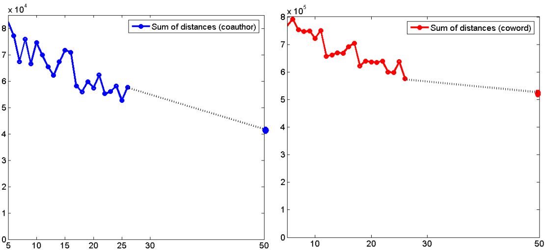
Figure 2. Sum of distance for k-means
