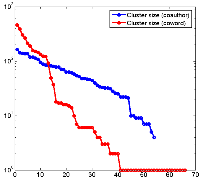
Figure 4. Cluster size (VOSviewer)
