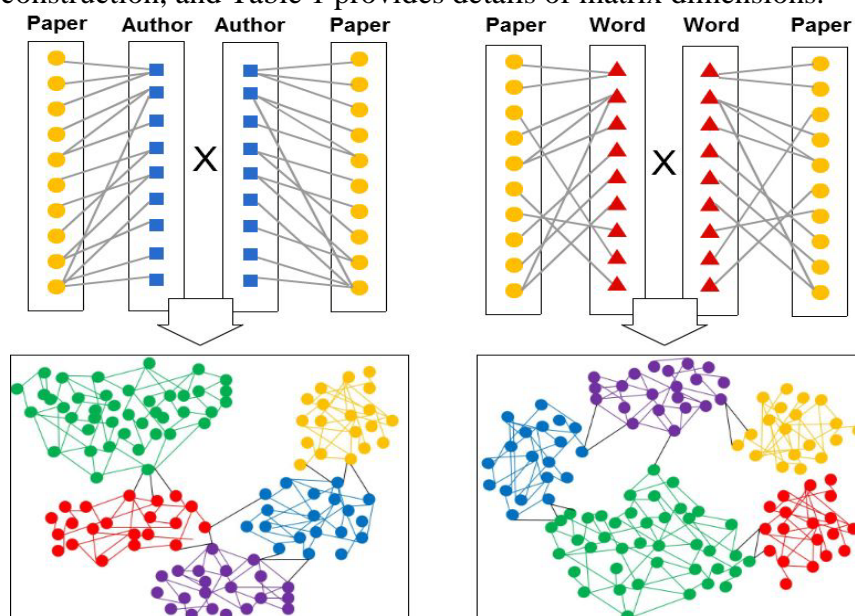
Figure 1. Network construction
