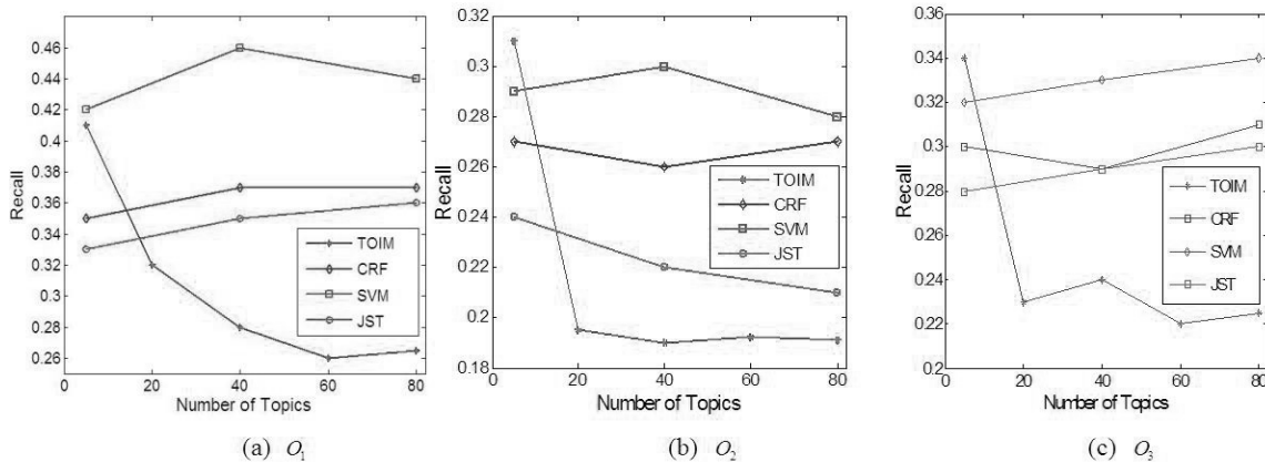
Figure 5: The recall of opinion inference for (a) O_1 , (b) O_2 , and (c) O_3 , using four algorithms: SVM, CRF, JST and TOIM. As the number of topics increases, the recall of TOIM decreases as well, since the likelihood of finding two users' opinions on the same topic decreases. By contrast, the recall of other three algorithms is not affected by topic numbers.
