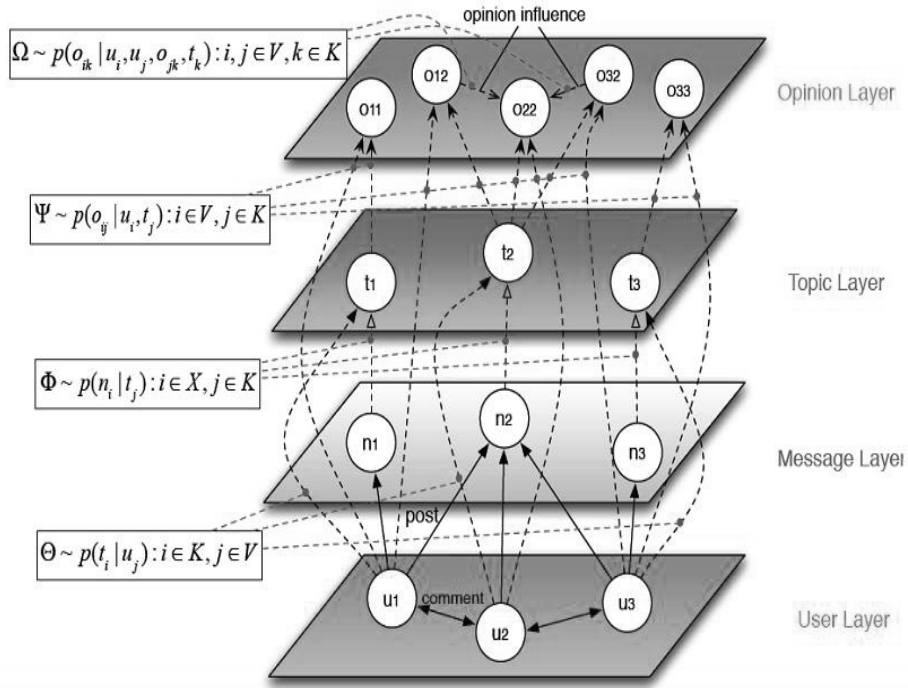
Figure 2: The framework of TOIM. There are four layers: user layer, message layer, topic layer and opinion layer. Users posted new messages and comment on others' messages. Some important entities occur in messages and belong to some topics. Given a new entity, some users' opinion about the entity is decided by both their historical opinion about the entity related topic and the opinion influence around this topic from his neighbors.
